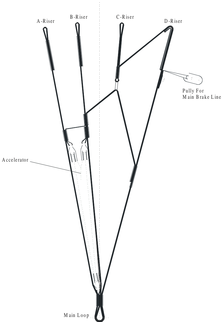
Illustration 2: UP Gambit Riser
