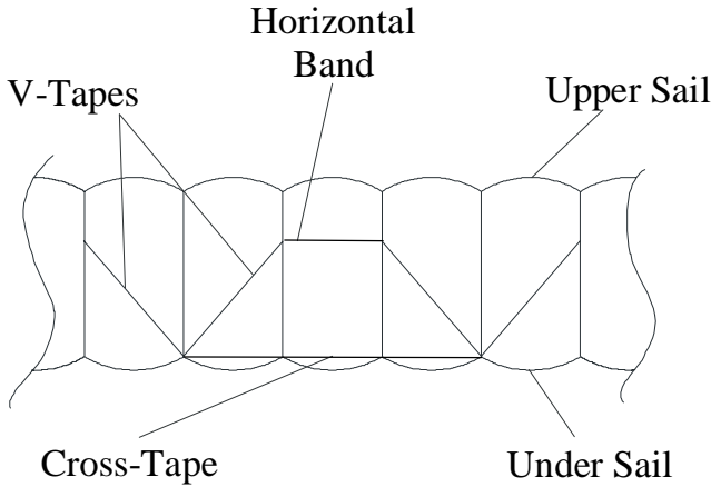
Illustration 1: Construction of the canopy
